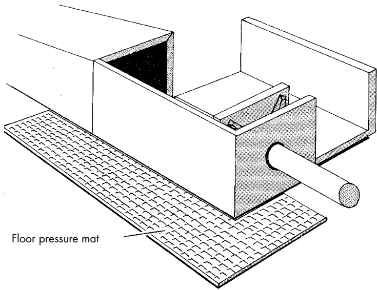
Fig. 4: Interlocked pressure-sensitive floor mat.
