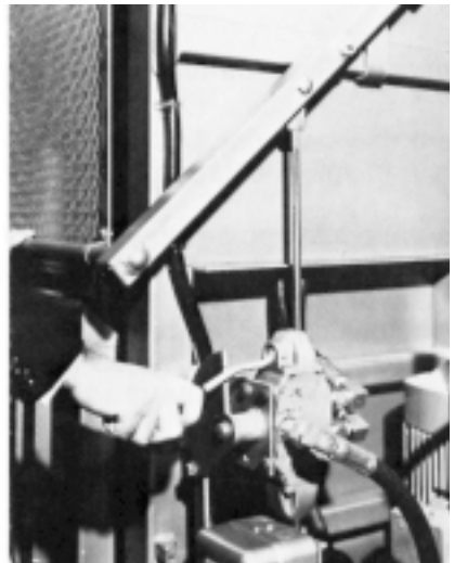
Fig. 7: Mechanical interlock (guard closed)
